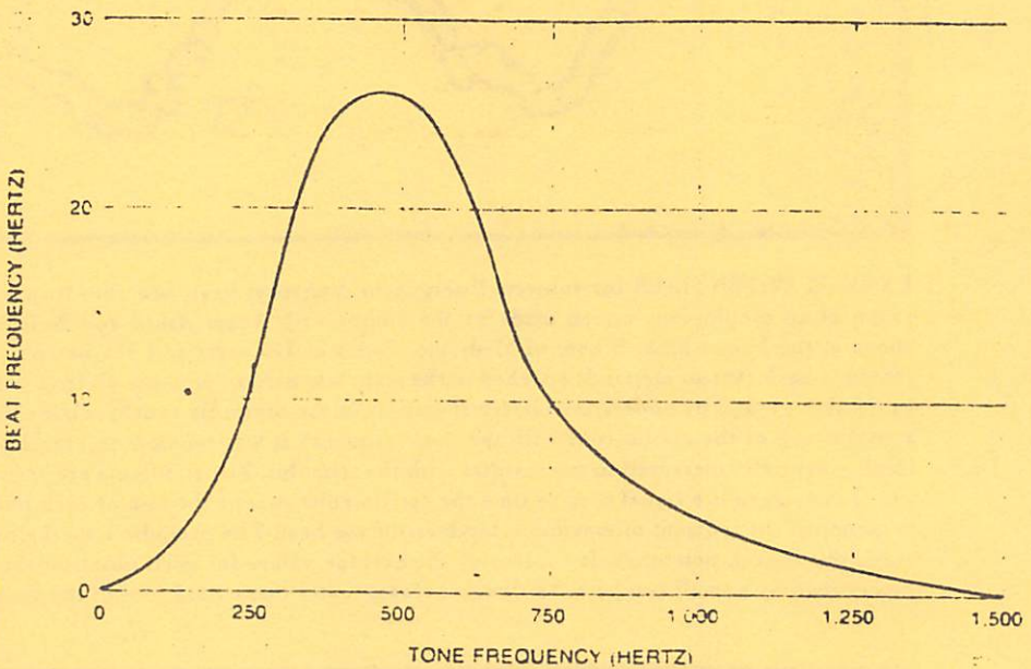
SPECTRUM OF BINAURAL BEATS was measured by J. C. R. Licklider, J. C. Webster and J. M. Hedlum. Rapid beats, up to about 26 per second, can be heard when the tones used to produce them are about 440 hertz. With tones of higher or lower pitch the maximum beat frequency declines. When the interval exceeds about 30 hertz, two tones are heard.
