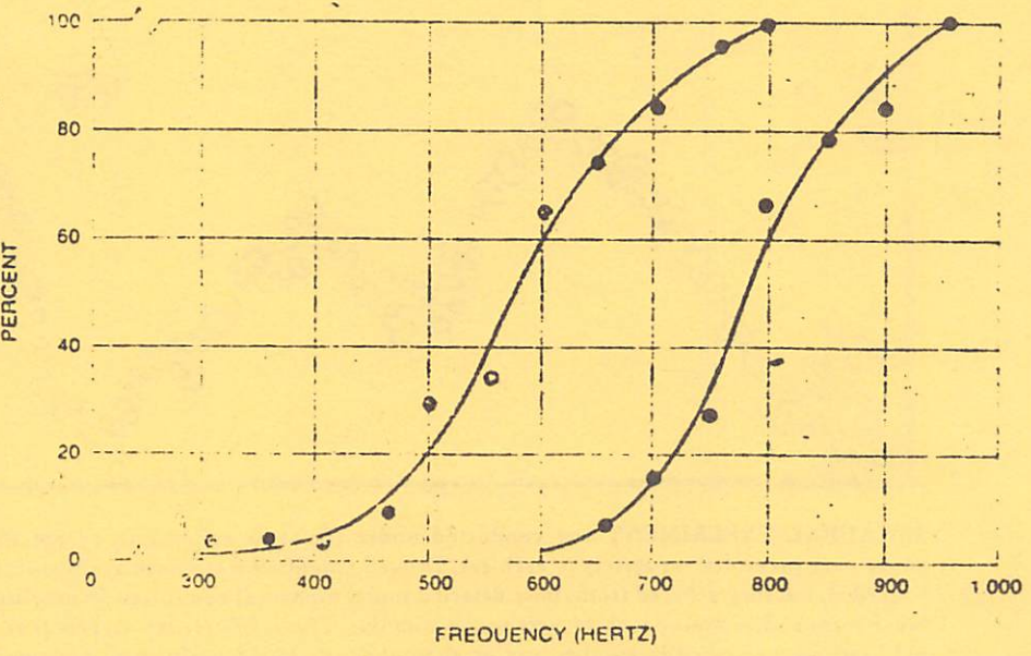
SEX RELATED VARIATION in the perception of binaural beats is plotted from data compiled by J. V. Tobias. As the pitch of the tones used to produce beats increases, both men (color) and women (black) cease to perceive them. Women, however, lose the ability at lower frequencies. Some female subjects also report variations during the menstrual cycle.
