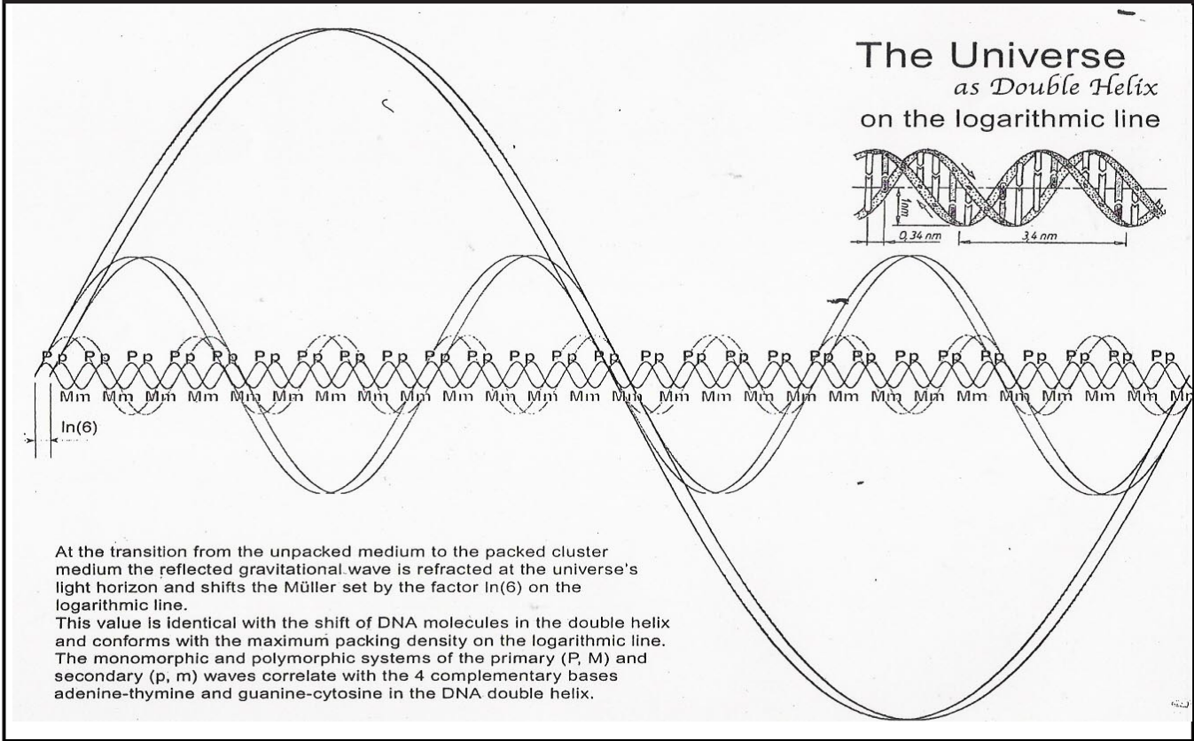
Figure 1. Structure of the Standing Gravitational Wave (SGW) of the Universe
