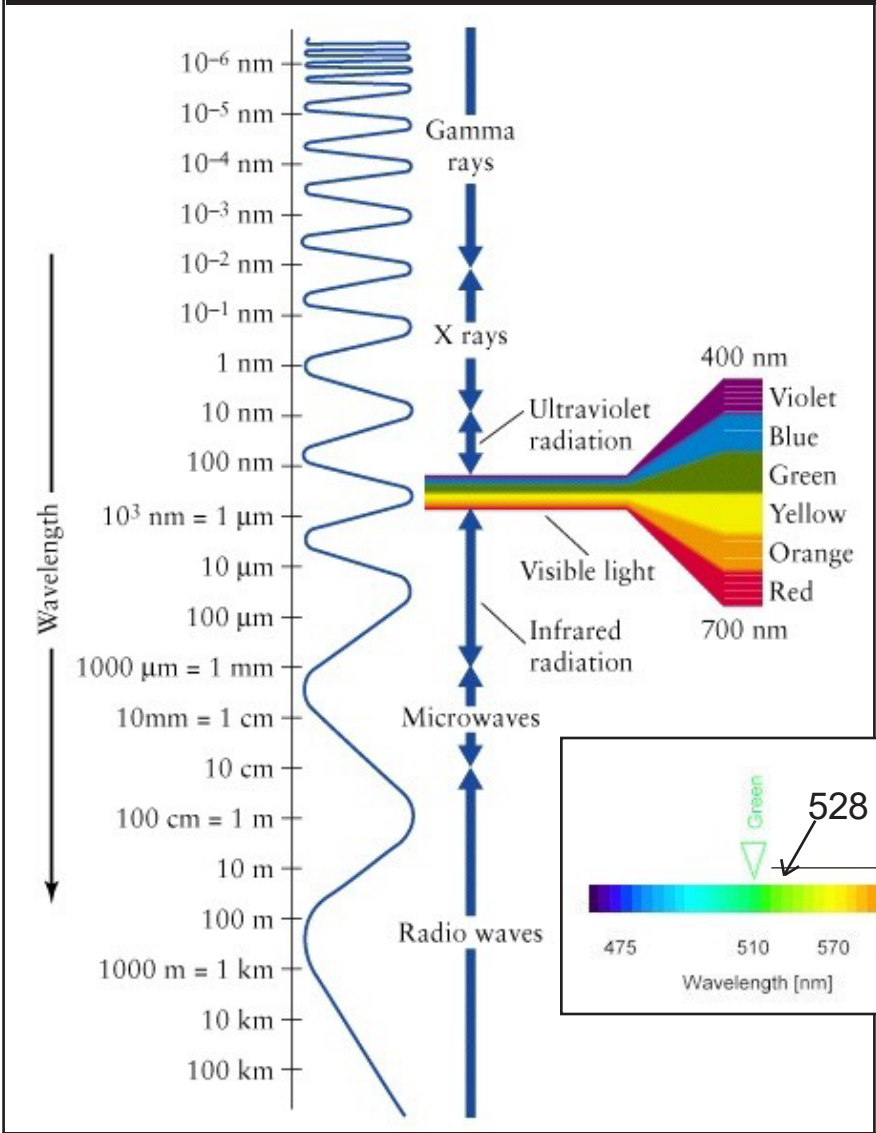
Figure 7. Electromagnetic Spectrum of Wave Frequencies
