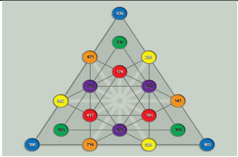
Fig.60. SolfeggioFrequencies'RelationshipsChart
